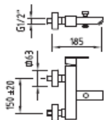
BAÑO-DUCHA BATH-SHOWER BANHEIRA 96.853
