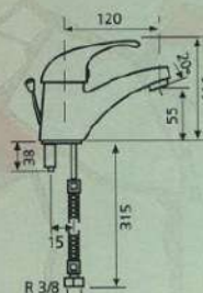
95010400 MONOMANDO LAVABO MITIGEUR LAVABO SINGLE HANDLE WASHBASIN MIXER
