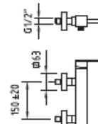
DUCHA SHOWER DUCHE 96.854
