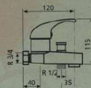
95040400 MONOMANDO BAÑO MITIGEUR BAIN-DOUCHE SINGLE HANDLE BATH-SHOWER MIXER
